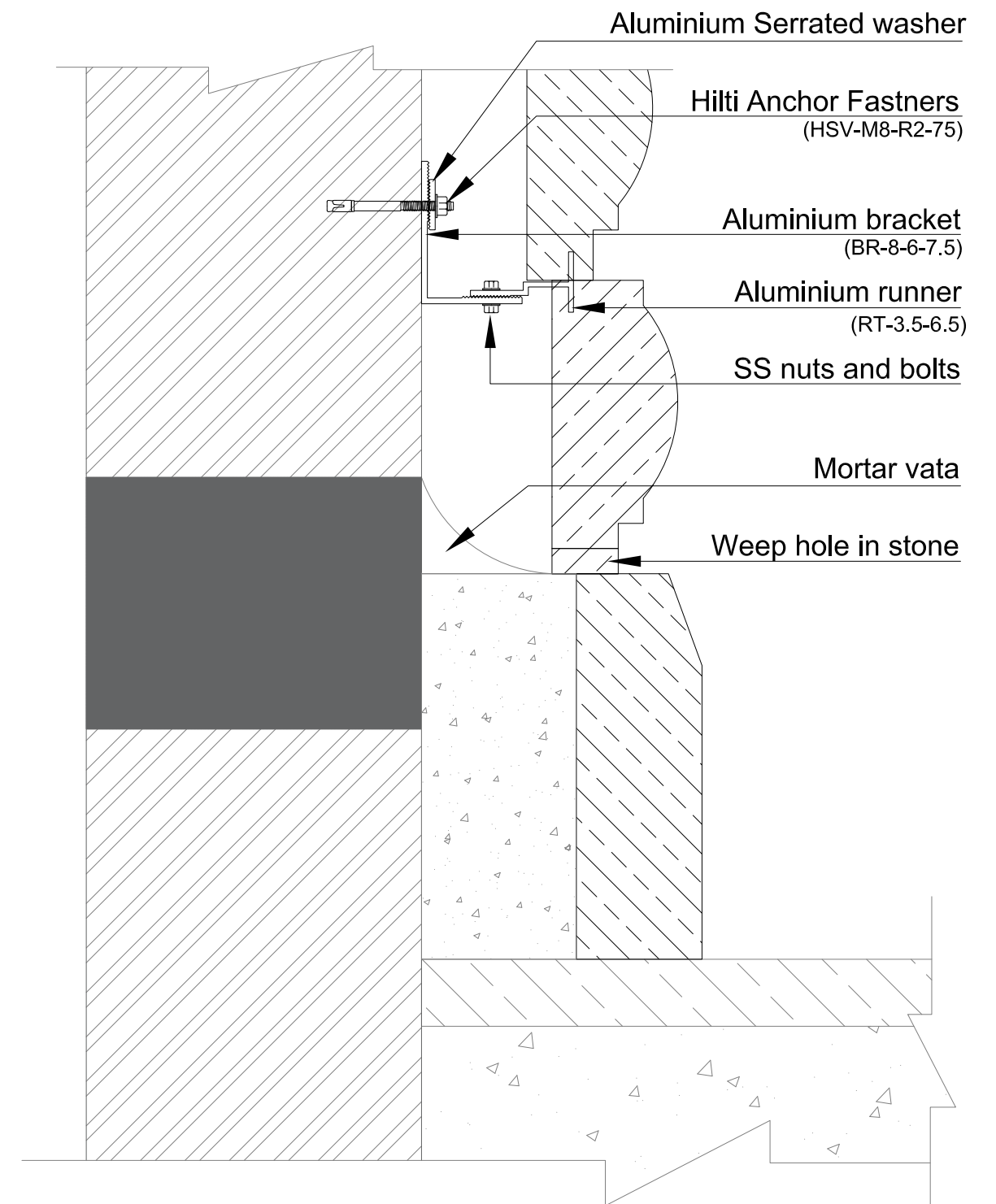
TYPICAL SECTION
