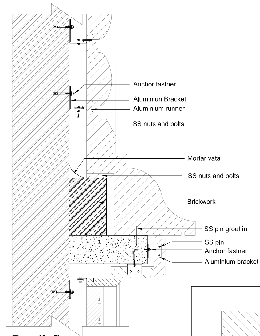
Detail-C
