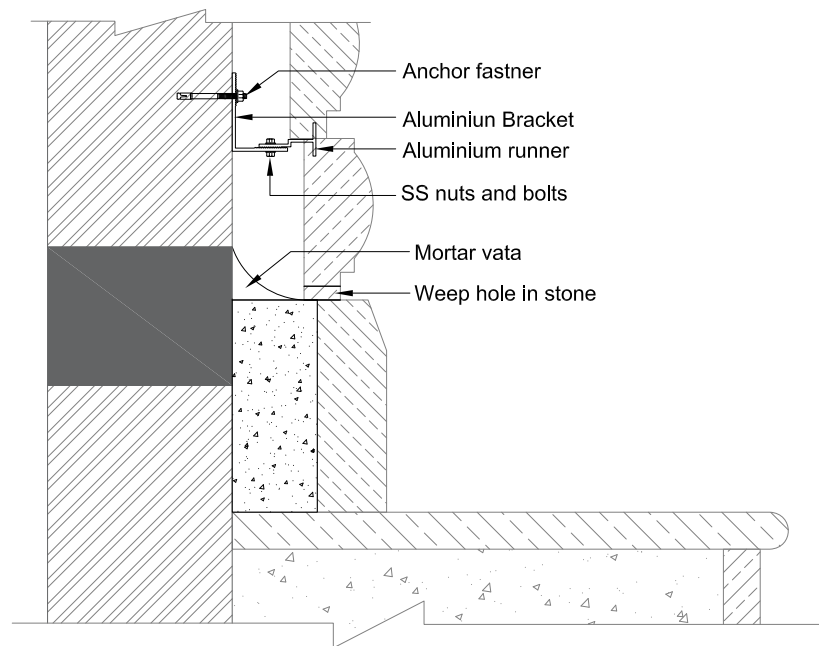
Detail-A
