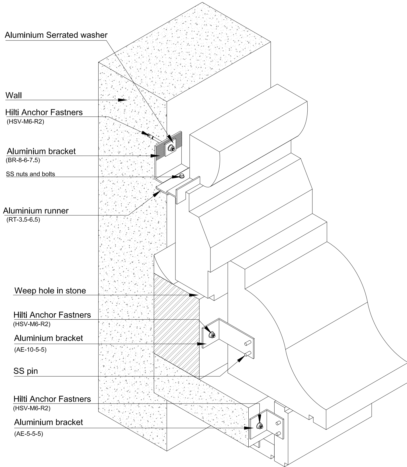
ISOMETRIC VIEW
