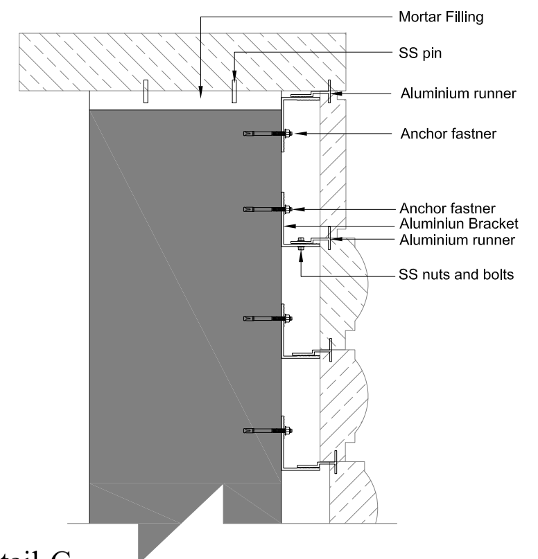
Detail-G
