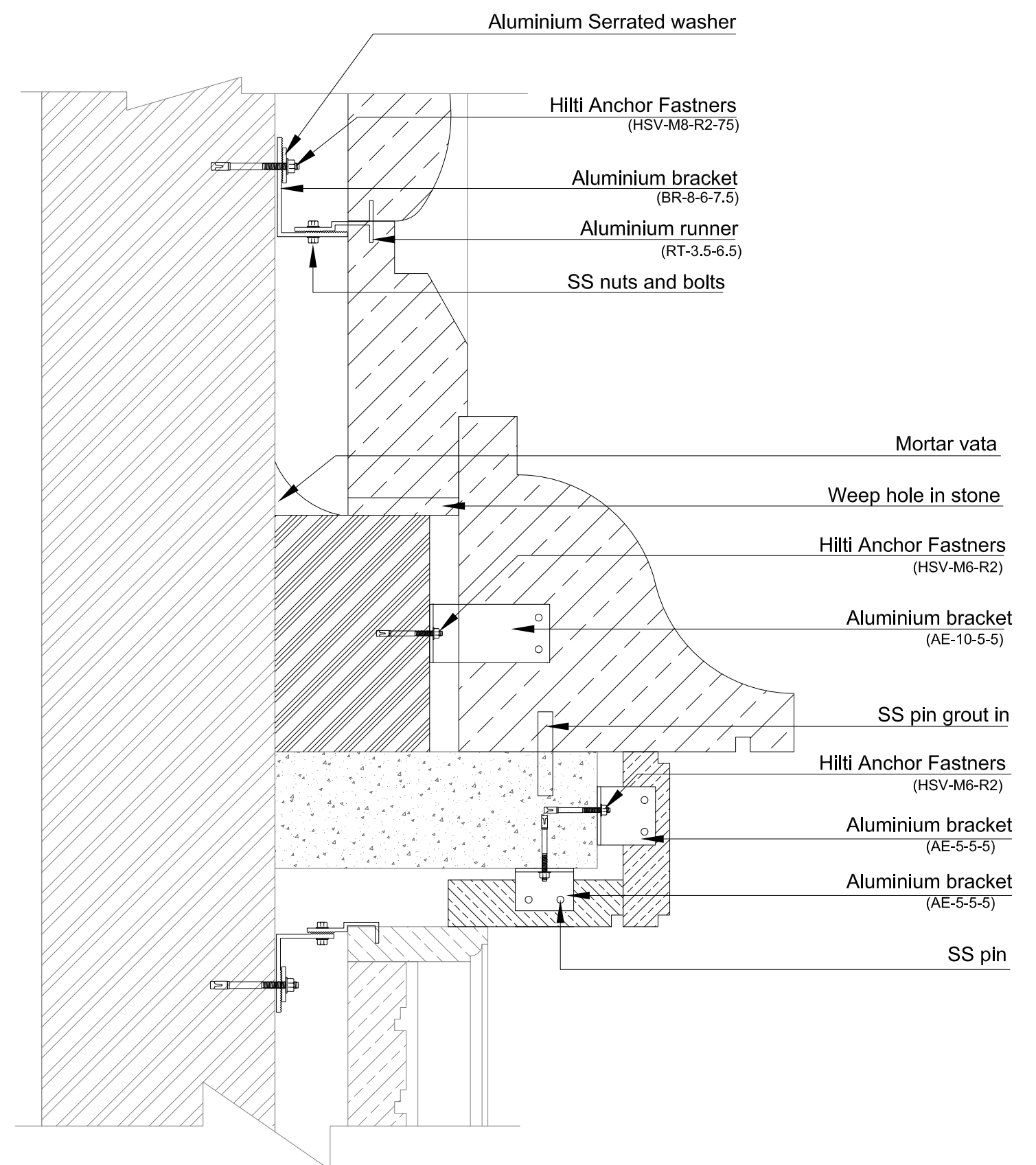
TYPICAL SECTION
