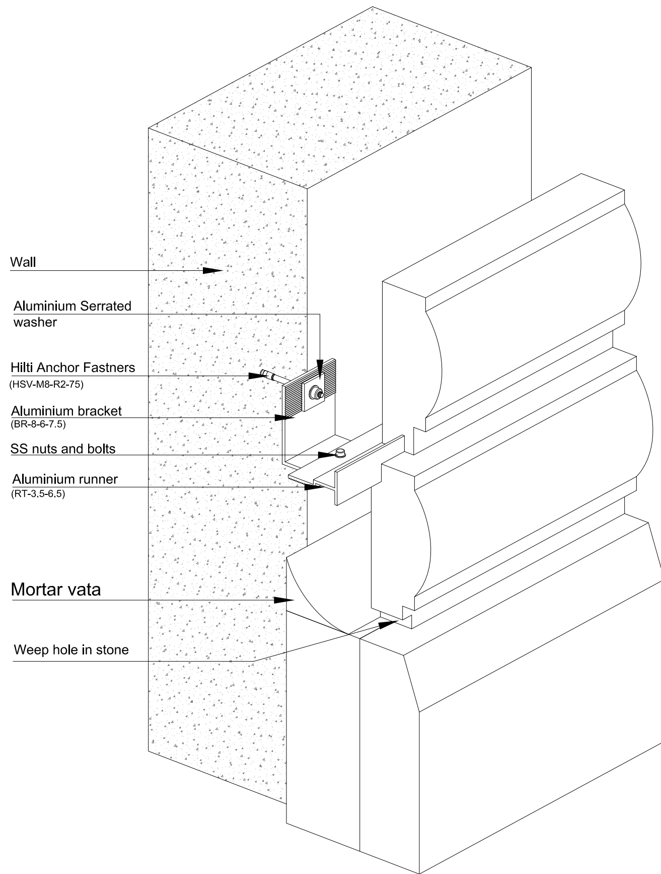
ISOMETRIC VIEW
